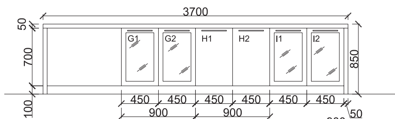
ELEVATION C
